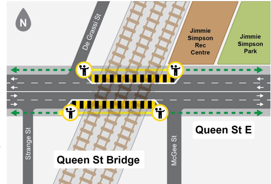
Debris Platform Installation and Bridge Deck Demolition
