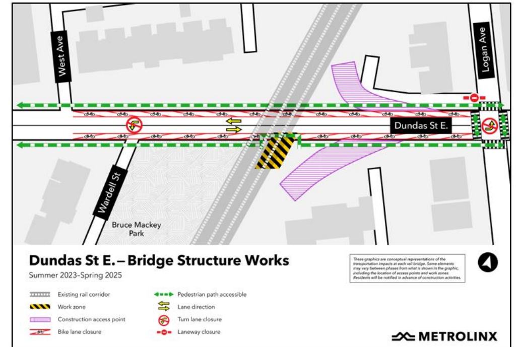
Figure 7 – Dundas Street Traffic Management during Bridge Abutment Works
