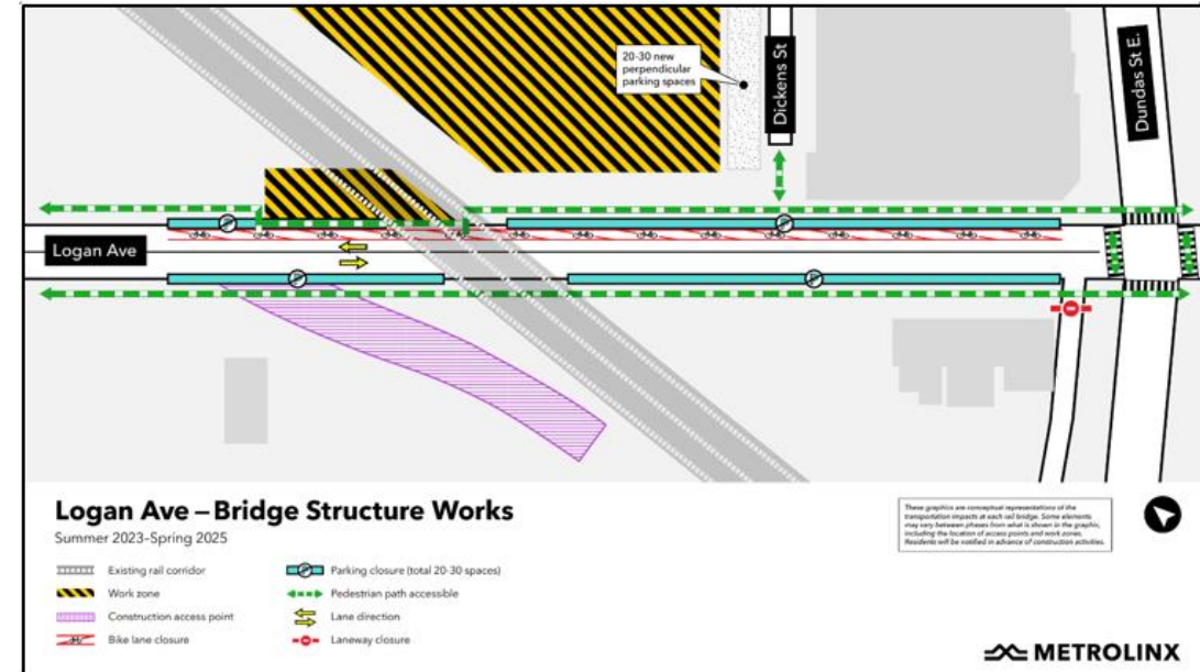
Figure 5 – Logan Avenue Traffic Management during Bridge Abutment Works Source: Metrolinx
